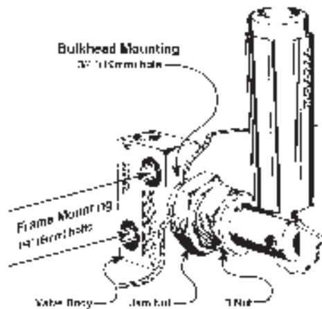
Diagram 1 - Mounting Diagram
